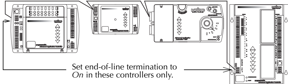
Illustration 2-10 End of line termination
