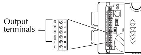
Illustration 2-6 Output terminals
