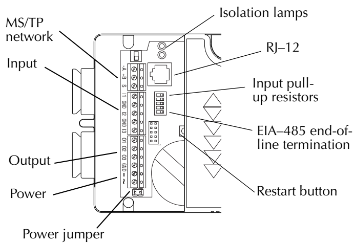
Illustration 2-4 Connection points inside wiring compartment
