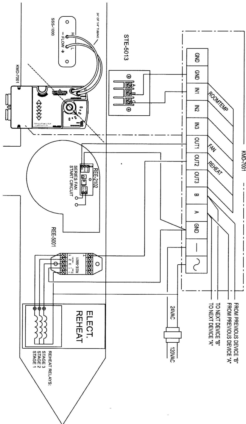
Illustration 13 VAV with three-stage electric reheat and series fan
